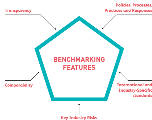
Figure 4: Benchmarking features
